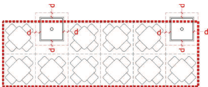
no hi ha protector, d = 20\text{cm}
